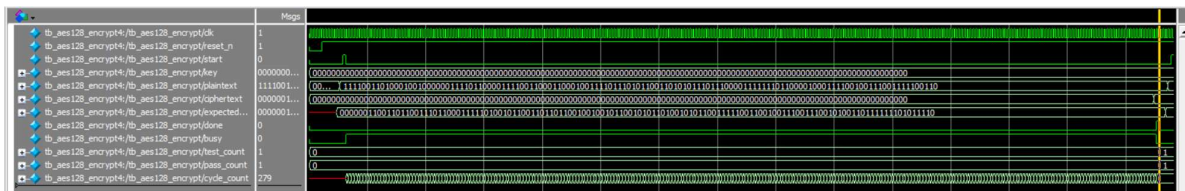
Figure 6.4: Optimized AES-128 Single Test Vector Verification Waveform
