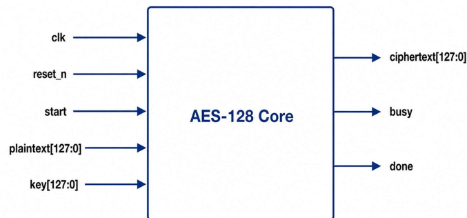
Figure 5.1: AES-128 Top-Level Interface Diagram
