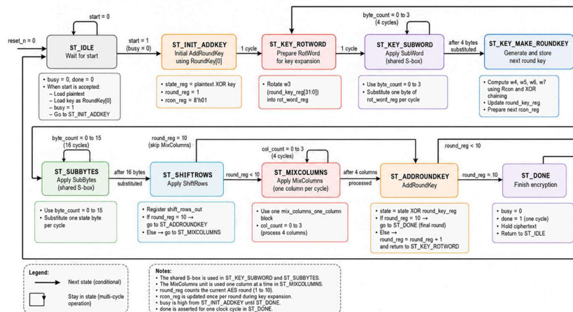
Figure 5.4 Optimized AES Controller – FSM State Diagram
