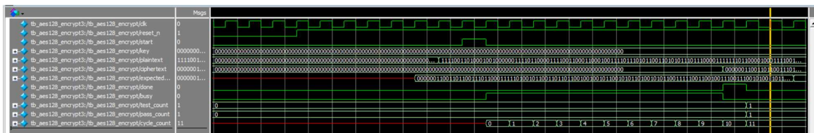
Figure 6.3: Baseline AES-128 Single Test Vector Verification Waveform
