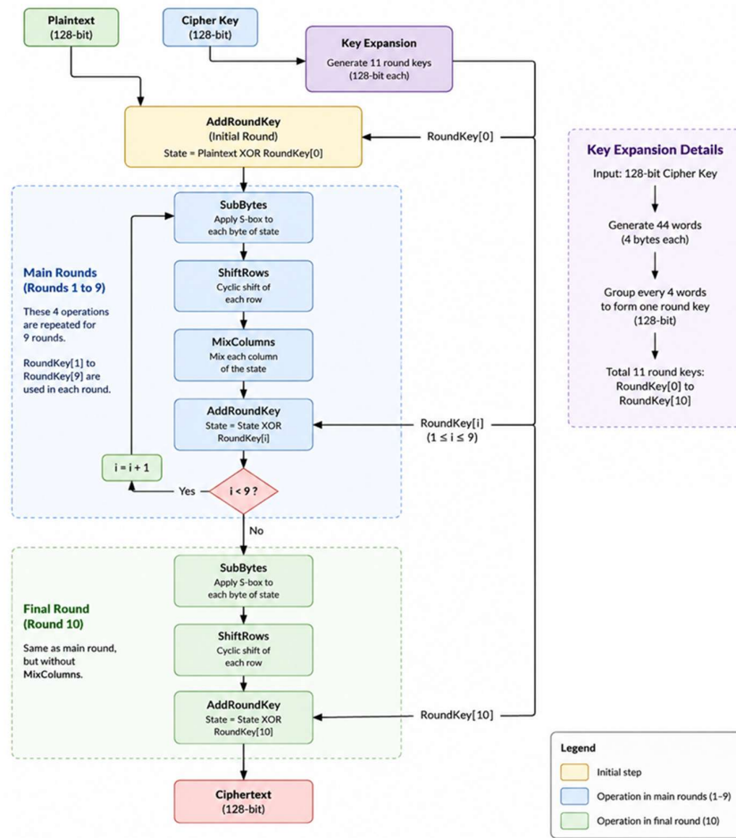
Figure 2.1: AES-128 Encryption Flow
